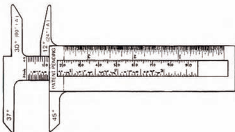
I.D./O.D. Angle Gauge Caliper
